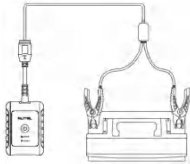
Figure 13-3 Connecting to a Battery
